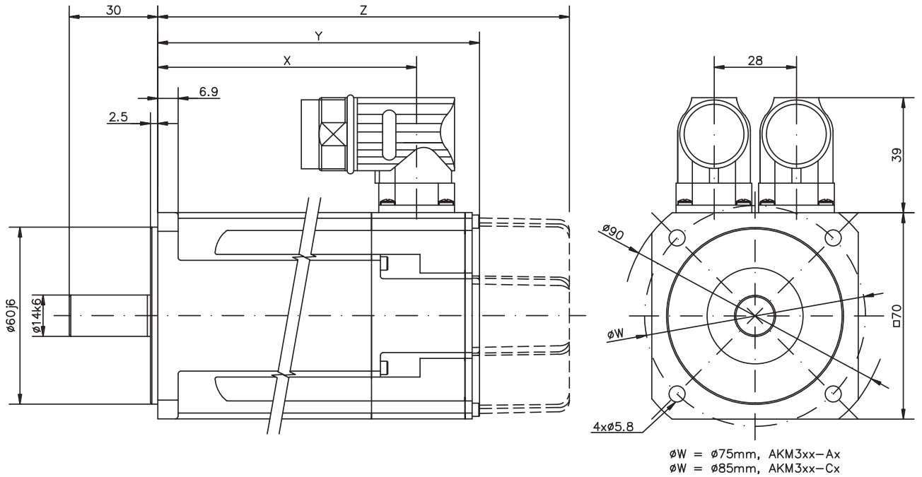
Option Keyway
