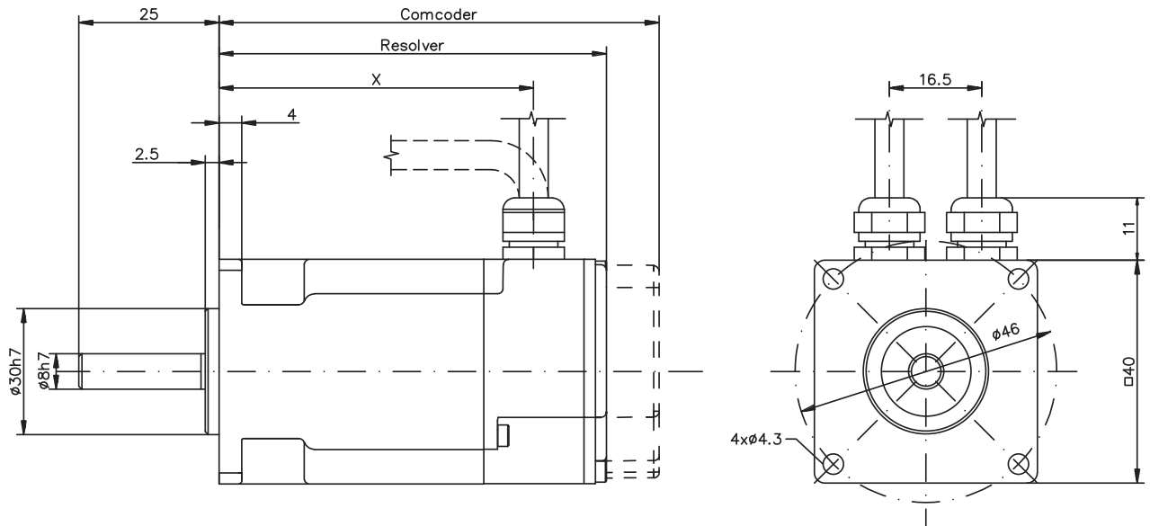
Option Keyway
