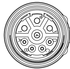
SINE 34-54774 CONNECTOR (FACE VIEW)
