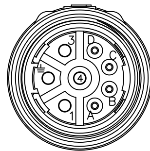
FACE VIEW
