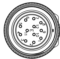
FACE VIEW
