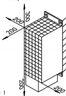
Admissible wall mounting Clamps down
