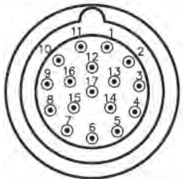
View: solder side of the motor connector.
