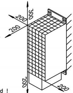
Admissible wall mounting Clamps down
