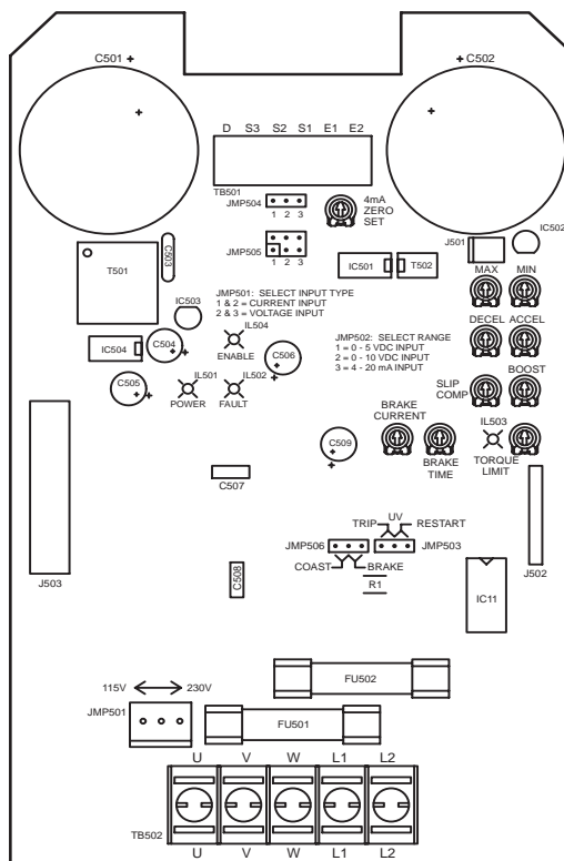
BVFD163 & BVFD163WD CIRCUIT BOARD LAYOUT
