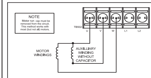
SINGLE-PHASE OPERATION (Configured for use with DIRECTION switch)
