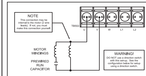
SINGLE-PHASE OPERATION (Motor with pre-wired capacitor)
