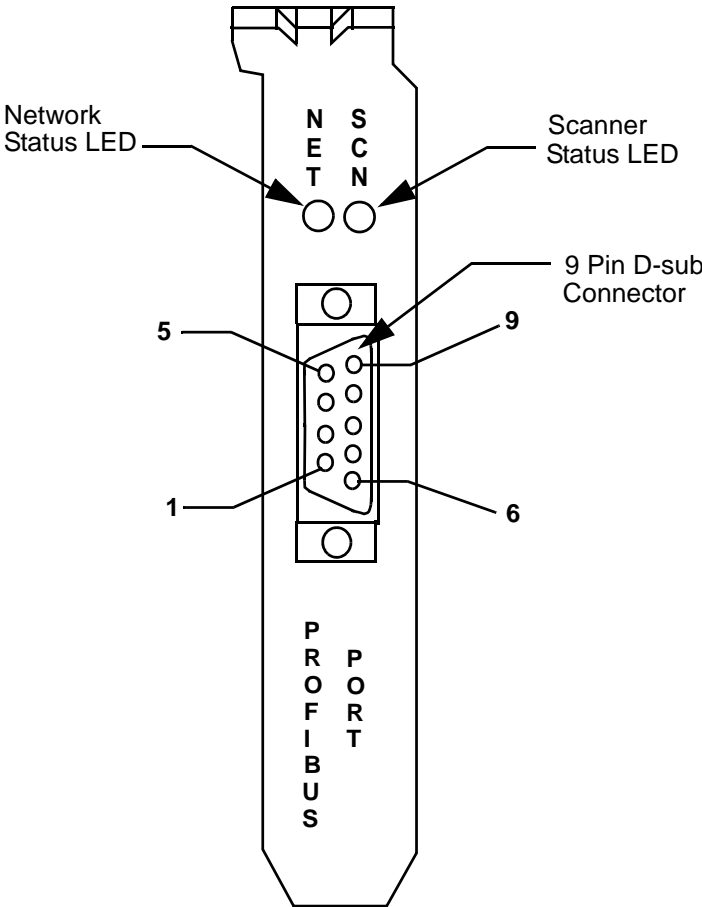
Figure 47: Profibus Port
