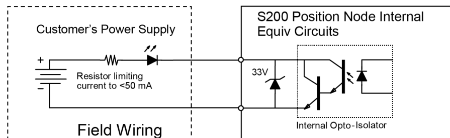
Wiring Discrete Output to LED or Opto Isolator
