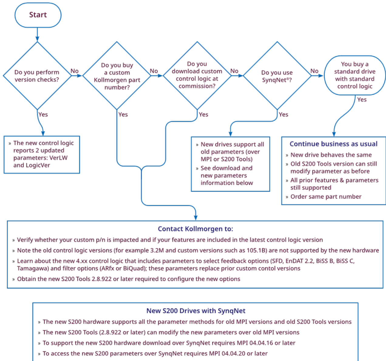
Figure C.1: Decision Tree – Does this HW update cause any customer change?
