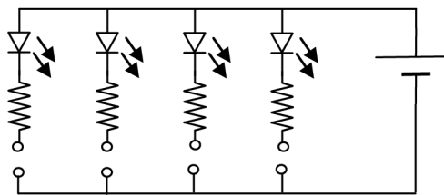
Figure 8.1 Common Rail Illustration
