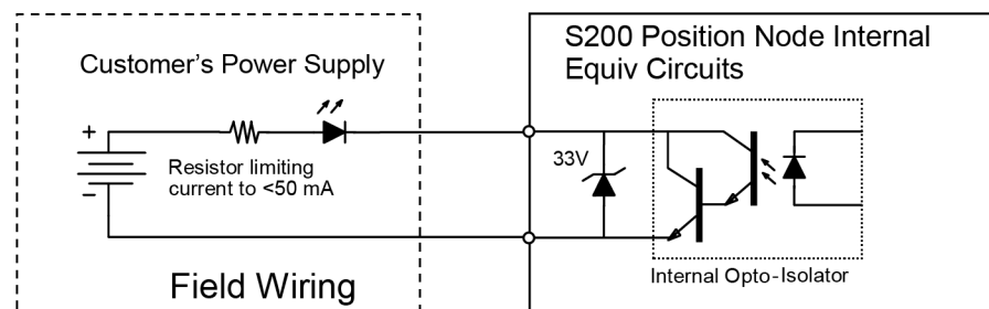
Wiring Discrete Output to LED or Opto Isolator
